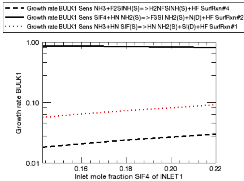
Figure 3 Steady-state Thermal CVD—Growth Rates
